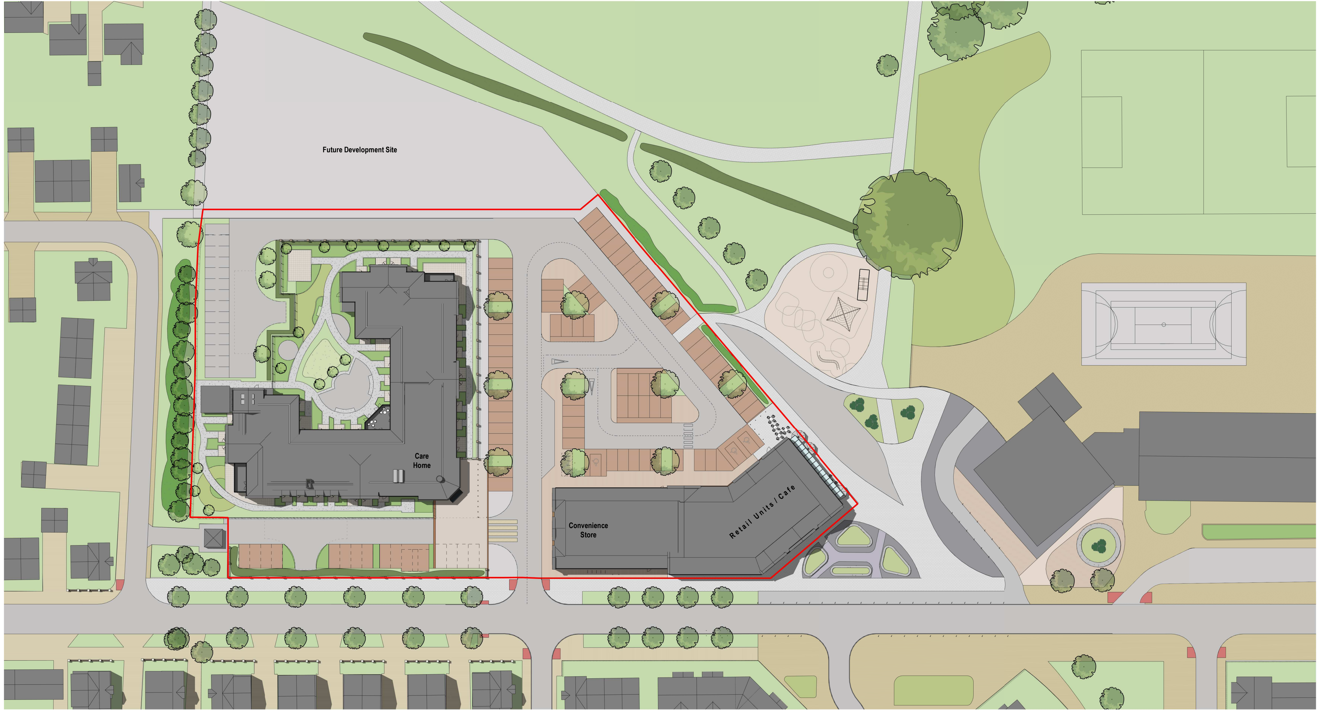
1 Site Plan Proposed Roof Plan 1 : 500
